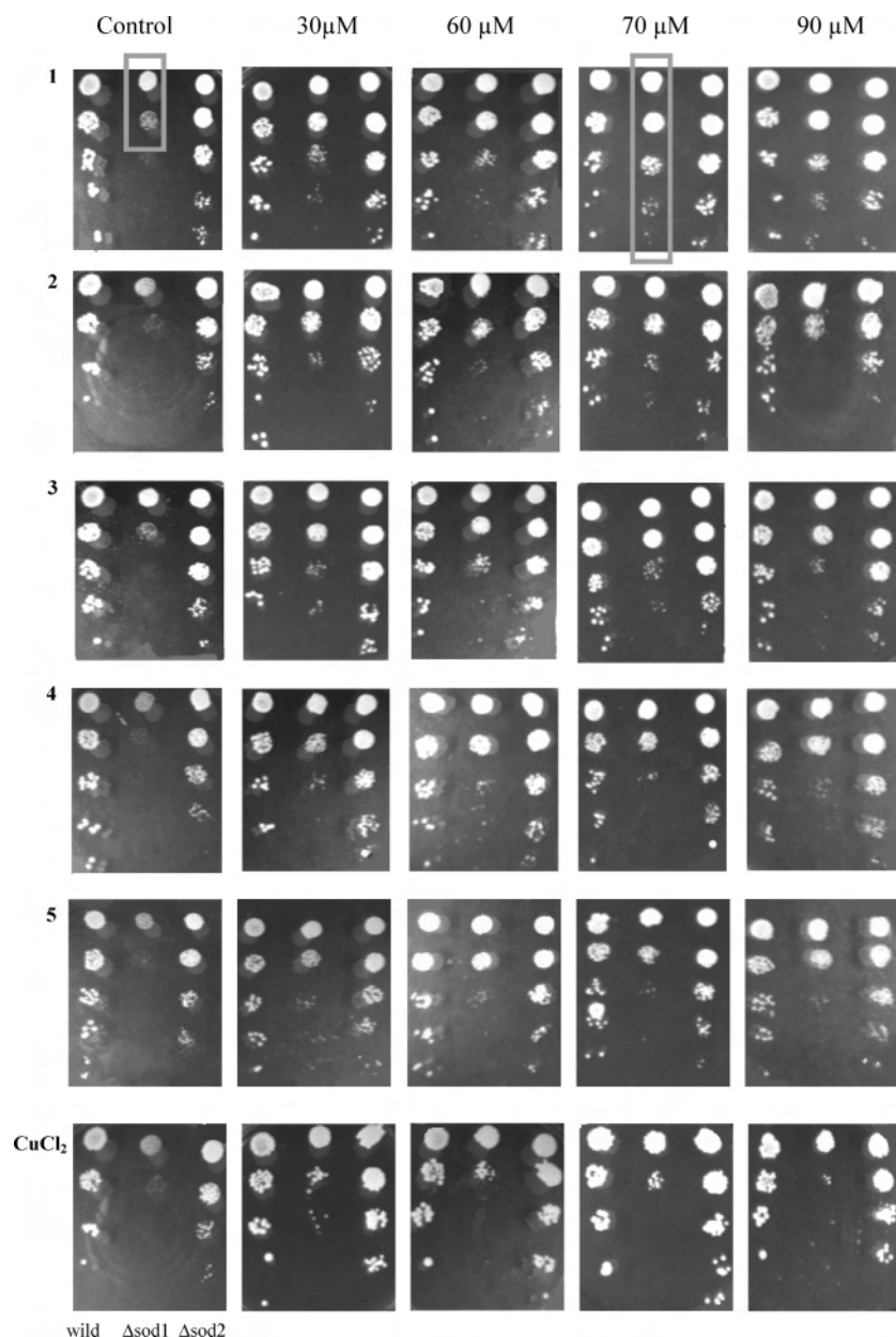
Figure 4. Effect of complexes 1–5, and \text{CuCl}_2 on the growth of the Saccharomyces cerevisiae against free radicals produced by respiration. In each panel the first column represents a wild strain; the second column represents the \Delta\text{sod1} mutant; the third column represents the \Delta\text{sod2} mutant. In each column; strains are shown at decreasing dilutions: 10^{-2} , 10^{-3} , 10^{-4} , 10^{-5} , and 10^{-6} .
