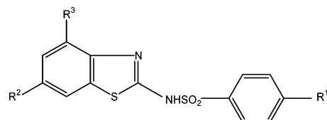
Scheme 1. N -Substituted Sulfonamides
