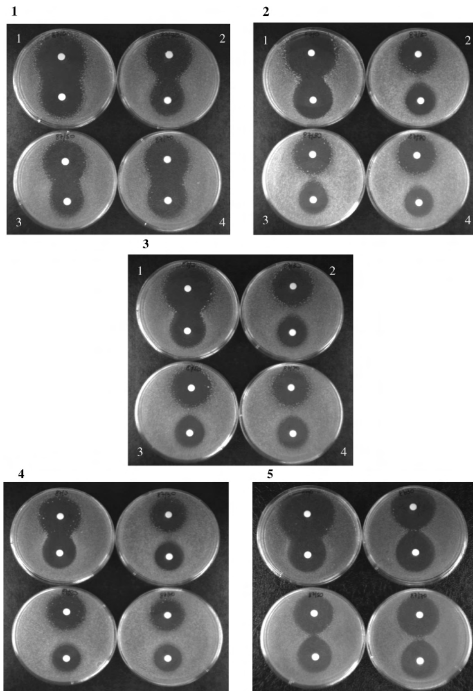
Figure 5. Effect of complexes 1–5 on the growth of the \Delta sodI mutant against free radicals produced by menadione (paper disk at the top of each Petri dish) and H_2O_2 (paper disk at the bottom of each Petri dish). For each photograph, 1 is the control; 2 is the 30 \mu M complex; 3 is the 50 \mu M complex; 4 is the 70 \mu M complex.
